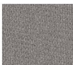
Occurrence CSE2
